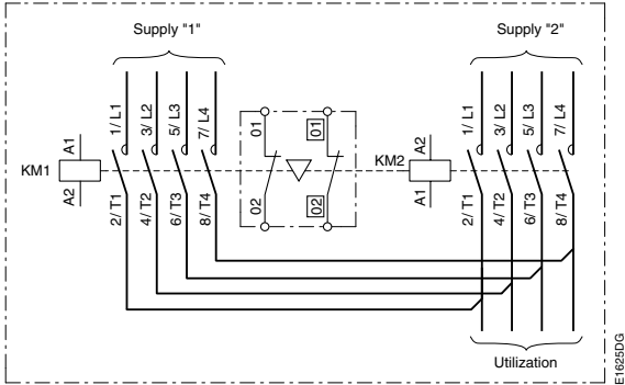
Power circuit
