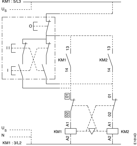
Remote control
